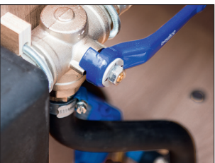
Direct drain – grey-water tank bypass (not for Royal 600 TDL, standard on Imperial)
