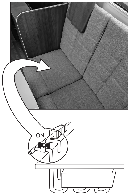
Diagram of valve location in the convector system. (Only models with the fresh water tank under the floor.)
